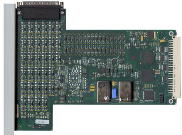
3126 32-Ch Analog/Digital Input Card
